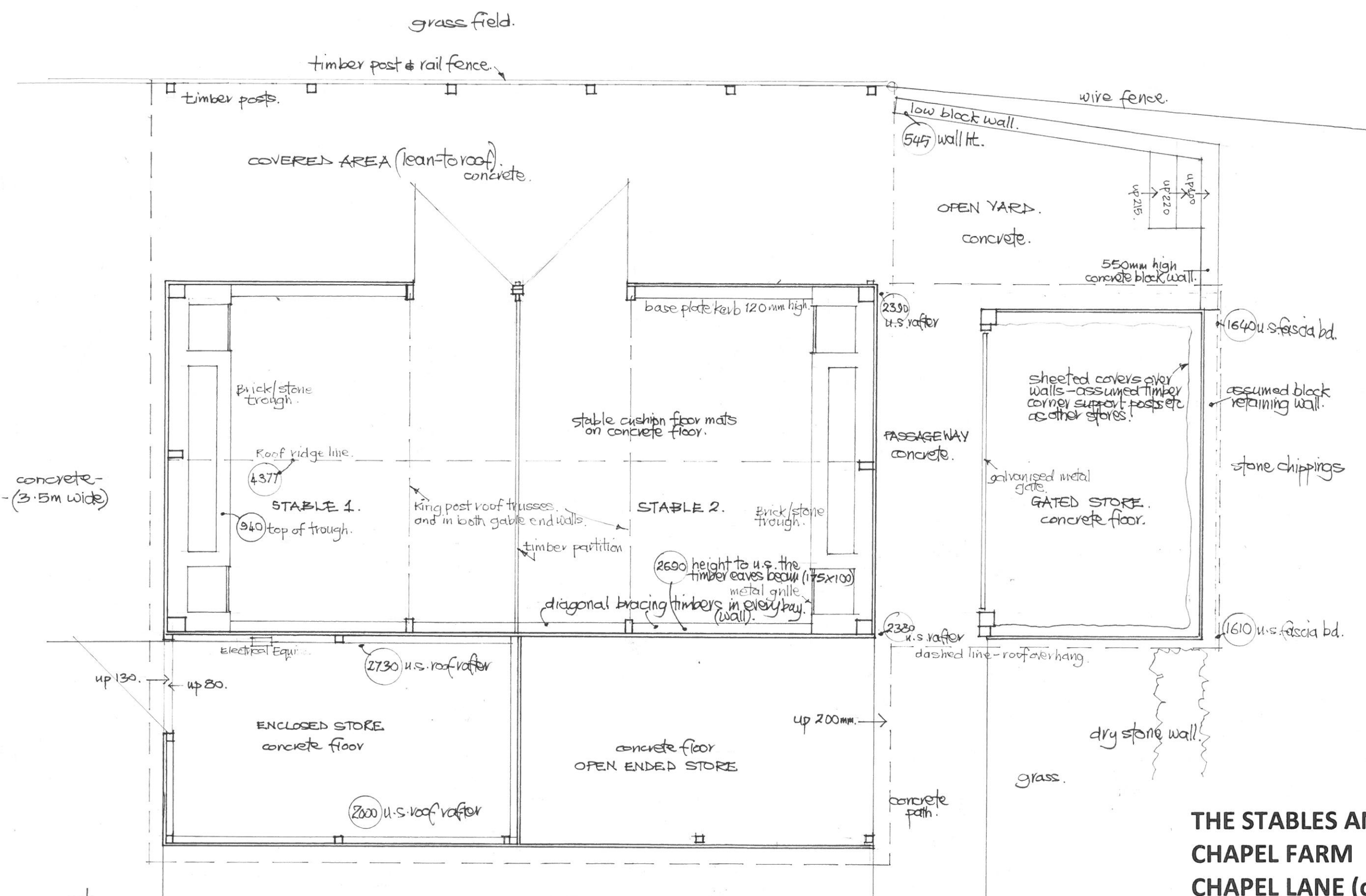
FLOOR PLAN - AS EXISTING SCALE 1:50 @ A3 DRAWING NO. CF.E /2020 / P1 DATE : AUGUST 2020.
