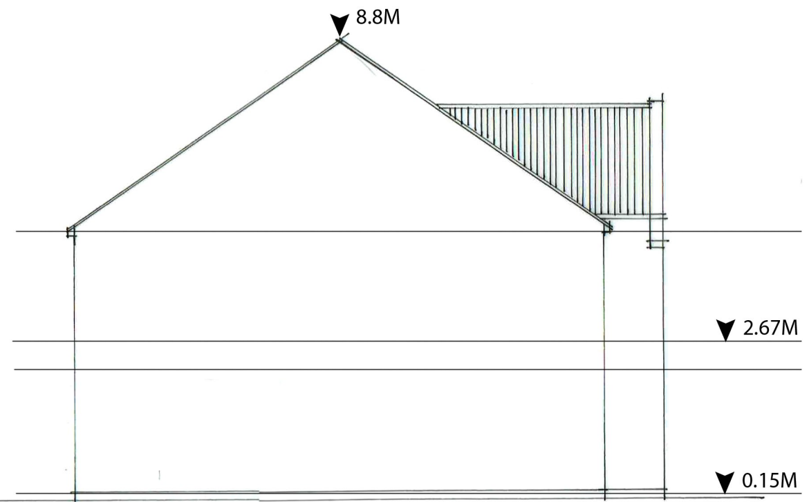
Ceiling and Ridge Heights
