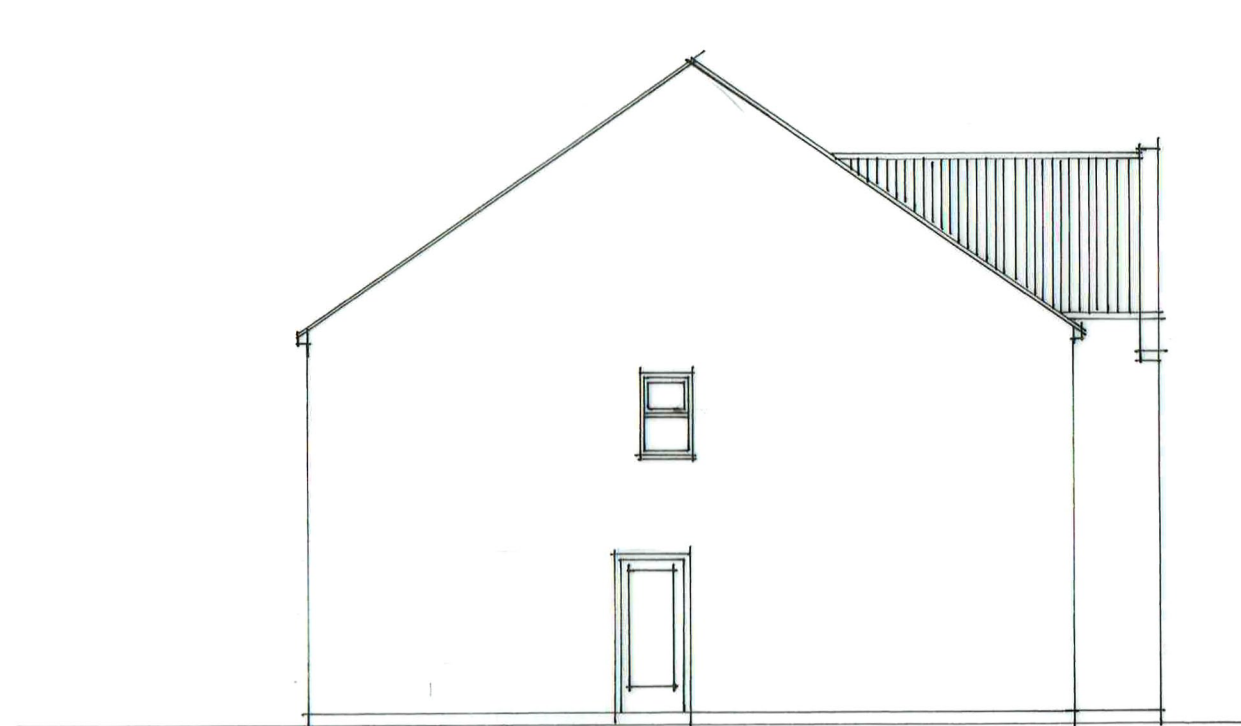
North Elevation (South mirror)
