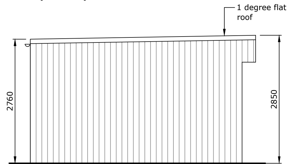
Rear (West) Elevation
