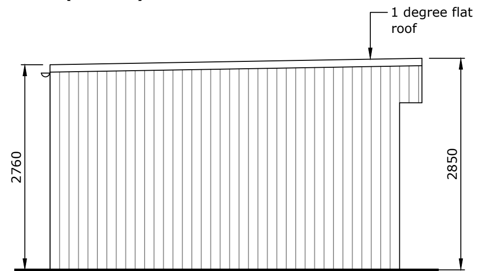
Rear (West) Elevation
